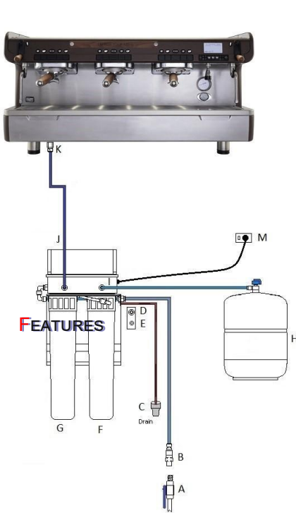
QuadRO H202 Installation Diagram
