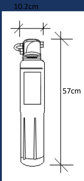
XP195 hard scale treatment system and replacement cartridge
